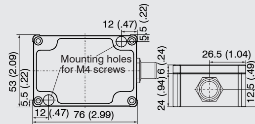
Fig. 2 Dimensional drawing, dimensions in mm (inches), not to scale
