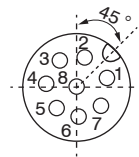
Fig. 3 View of solder pin side, 8-pin, A-coded, female connector
