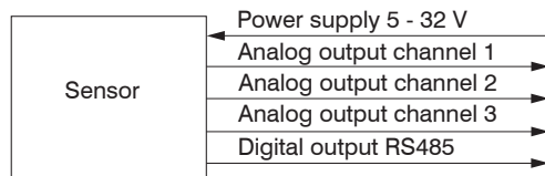
Fig. 4 Current and voltage output
