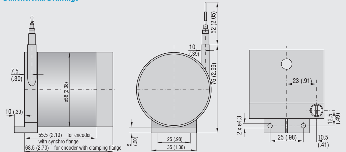
WDS-Z60-M series, dimensions in mm (inches)
