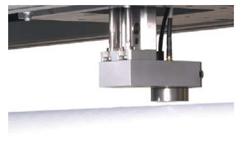
Non-contact, inline thickness measurement of plastic films
